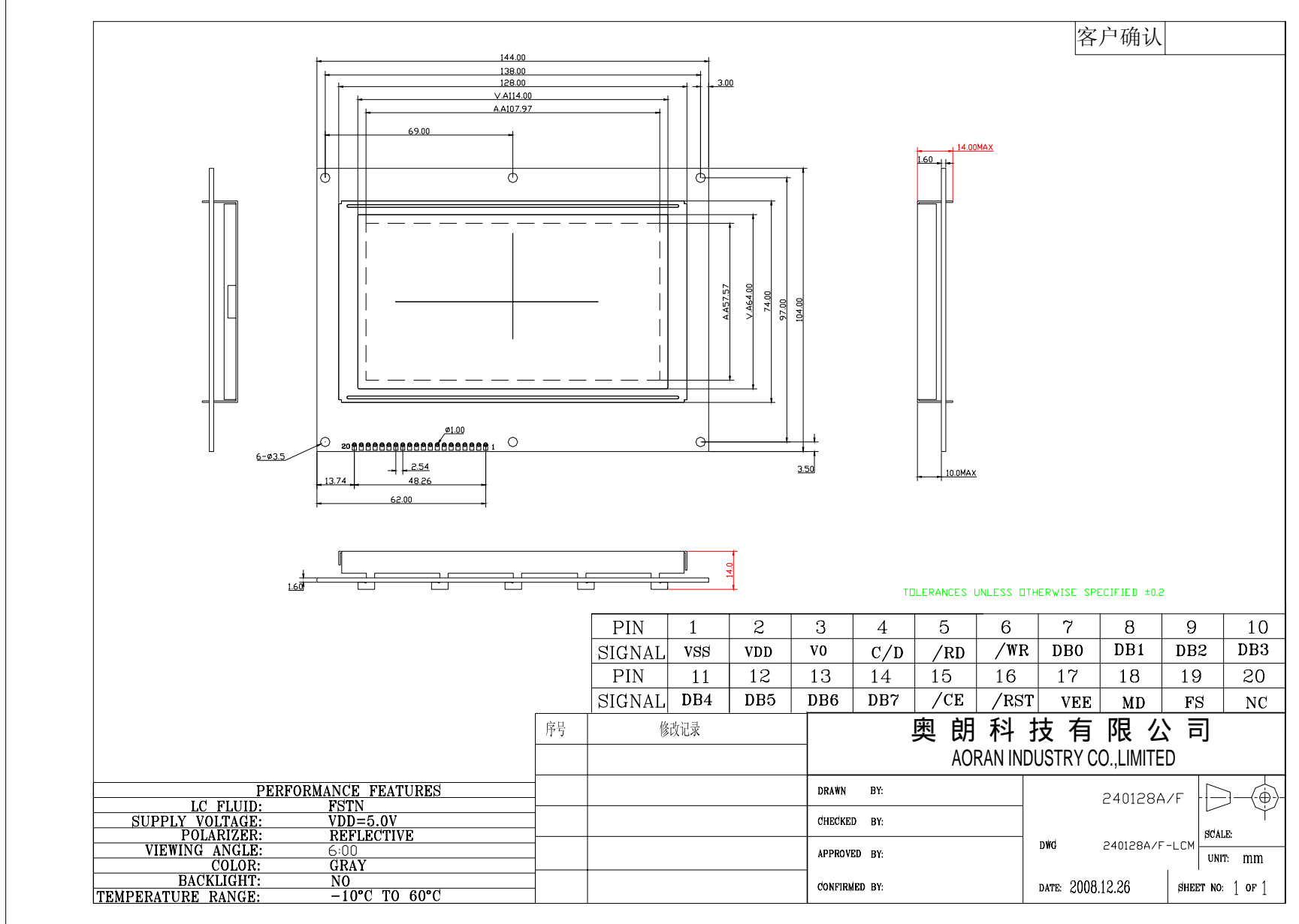
FIGURE 1. EXTERNAL DIMENSIONS
